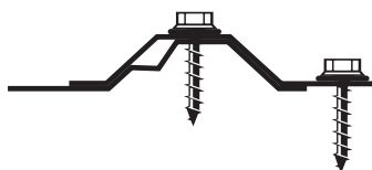
LAP DETAIL
